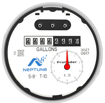
Figure 1: ProCoder™ Dial Face with Sweep Hand
